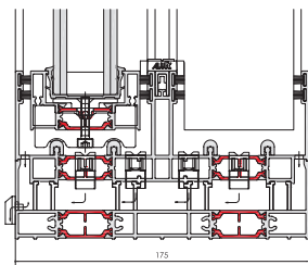
Sill Detail of Flush Threshold Configuration
