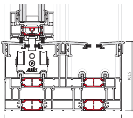
Bottom Section of Flat Sill configuration
